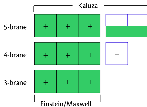
Figure 11 • A context for Kaluza
