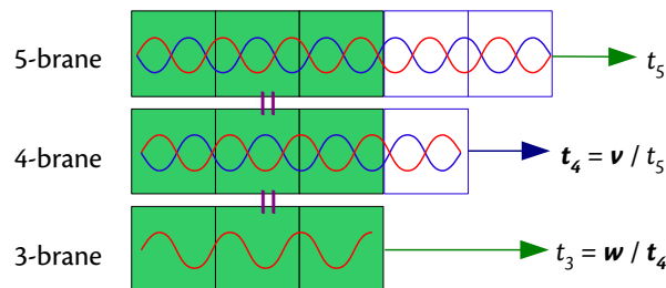
Figure 13 • The domain of the wavefunction
