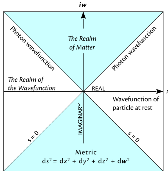
Figure 5 • Minkowski 4-space
