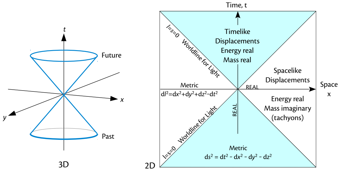
Figure 2 • Minkowski spacetime
