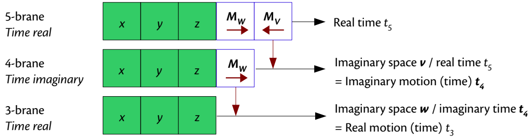
Figure 9 • Time and motion in the three branes
